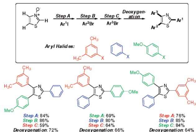
Scheme 1. Stepwise C2-C5-C4 Thiazole Arylation a
