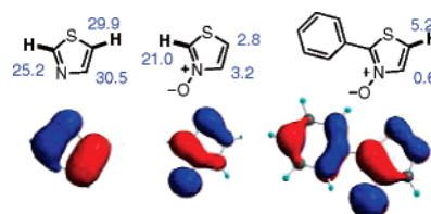
Scheme 2. HOMO for Thiazole and Thiazole N -Oxide Substrates a
